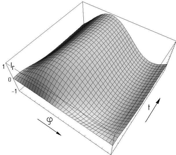
Fig. 3. The transient response of the variance of the induction currents distribution in the induction motor rotor under discontinuous variation of rotation speed.
