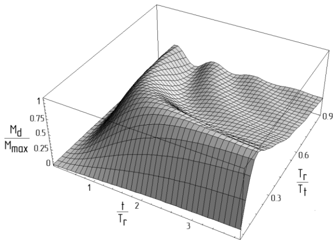
Fig. 4. The analytical array of transient response of the decelerating torque for different ratios of rotor characteristic time T_R and transportation time T_T .
